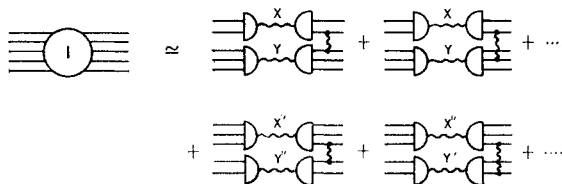
FIG. 8. The "pole approximation" for the irreducible kernel I(W) . We only keep those terms arising from simultaneous bound states of subsystems X, Y or X'Y' . The horizontal wavy lines represent the "propagators" [W+B]^{-1} , and the small semicircles indicate the wave functions of the various bound subsystems. The notation + \dots means that there are a few other terms arising from different ways that interactions V_{ij} can link the two subsystems.
