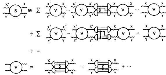
FIG. 9. The distorted wave approximation for the S matrix of the process X+Y \rightarrow X'+Y' , derived by stringing together any number of I 's from the first line of Fig. 8, and then continuing with a string of I 's from the second line of Fig. 8, with a single overlap integral between. Again, the notation + \dots indicates a few additional terms arising from other V_{ij} that can link the two subsystems.
